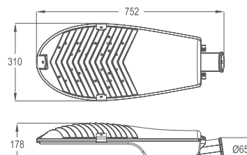
SDQ-M 100W / 120W
